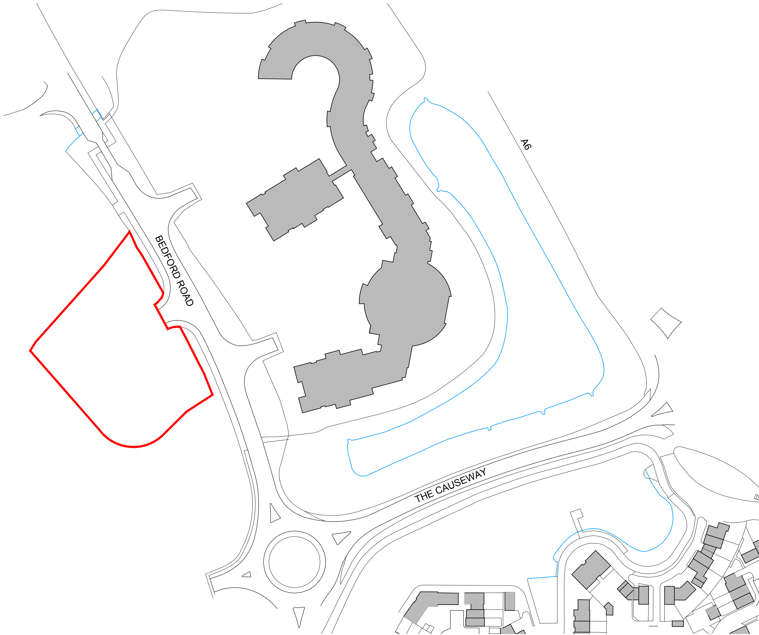
EXISTING - SITE LOCATION PLAN
